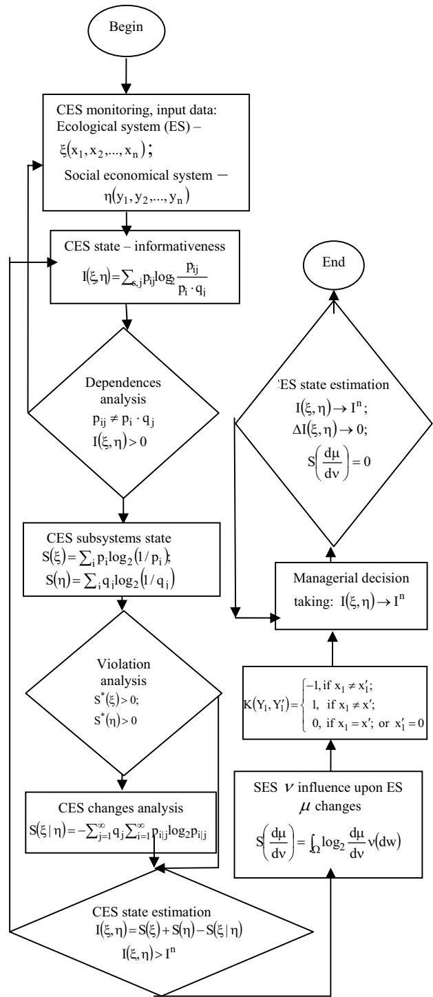
Fig. 1. CES state estimation scheme in the form entropy and comparator K: \xi is probabilistic observation (x_1, x_2, \dots, x_n) with probability (p_1, p_2, \dots, p_n) ; \eta is probabilistic observation (y_1, y_2, \dots, y_m) with probability (q_1, q_2, \dots, q_m) ; p_{ij} is probability of interaction of operation \xi = x_i; \eta = y_j ; S is entropy of systems state; \mu is ecological changes to man-made v argument (in accordance with Radona-Nicodima) ( S_t w = w(t + \tau) ); I^n is unconfigured state, equilibrium position; \int is determination S provided that I^n = 0
