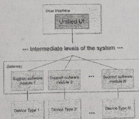
Figure 2 — Structure of the management system with abstraction
