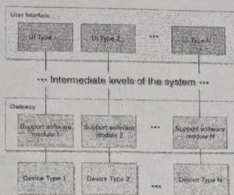
Figure 1 — Heterogeneous management system structure
