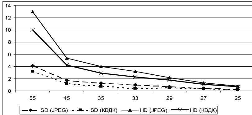
Fig. 2. The graphs of bit rate of frame PSNR for different spatial resolution
