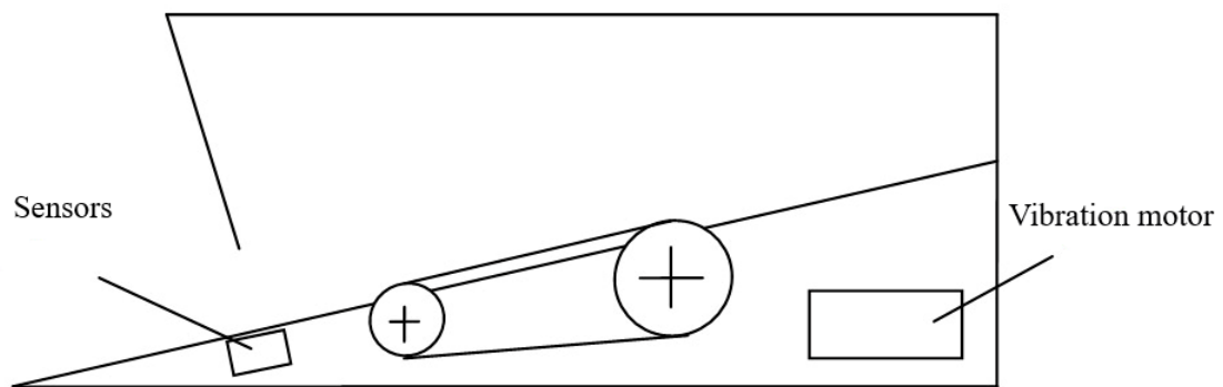
Figure 2: Kinematic diagram of the coin feeder
