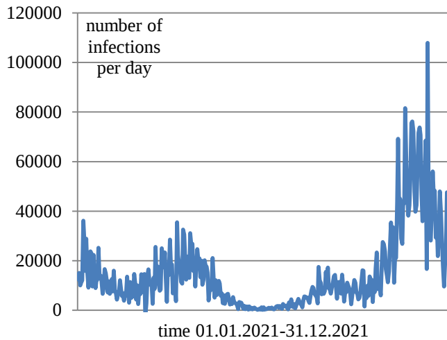
Figure 3: Evolution of infections per day in the Germany during the COVID-19 pandemic (selected time period)
