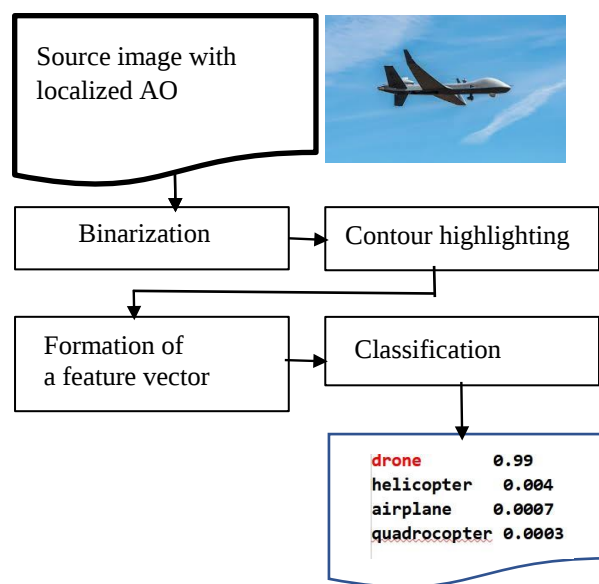
Fig. 3. Generalized block diagram of the air object type recognition procedure algorithm
