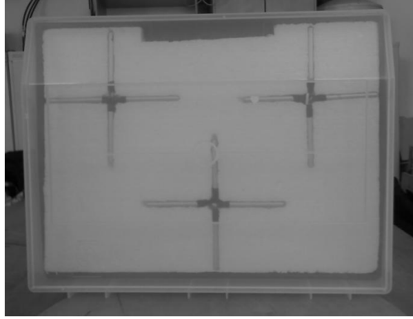
Fig. 3 – Real experimental polarization antenna for MIMO
