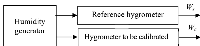
Fig. 1 – Scheme for comparing the reference hygrometers and hygrometer to be calibrated using a comparison device
