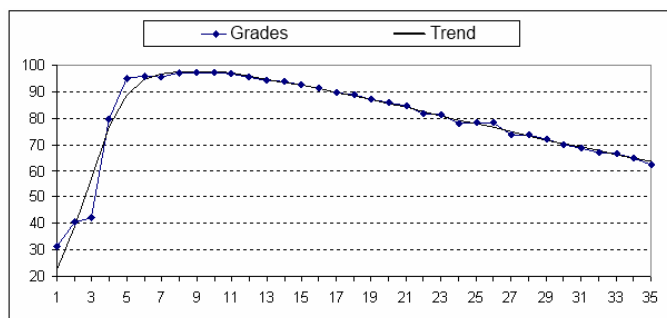
Fig. 5. Average estimates for the set {1,2,3,4}
