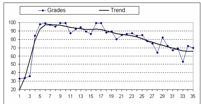
Fig. 3. Output range of estimates and its approximation
