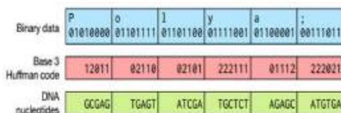
Fig. 2 - The process of converting a word to DNA nucleotides
