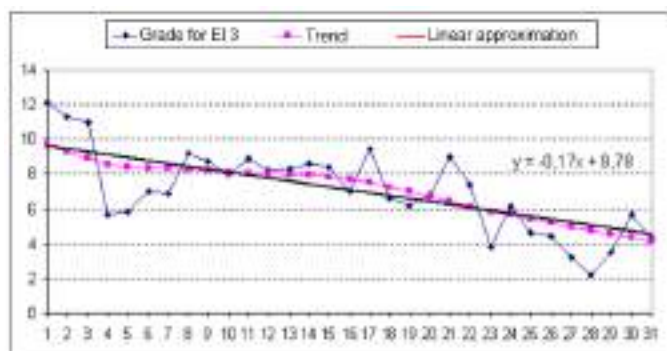
Fig. 7. Estimation of the effectiveness of EI 3
