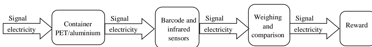
Figure 1: Automatic PET and Aluminum Packaging Device Operation Block Diagram
