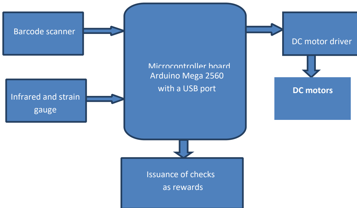
Figure 3: Diagram of a Signal Transmission in the Device Principle Simplified Version
