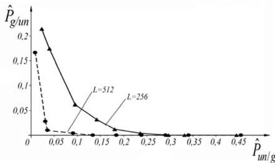
Figure 3 – Diagram of the exchange of quality indicators \hat{P}_{g/un} and \hat{P}_{un/g} for the recognition of given signals in the presence of unknown signals
