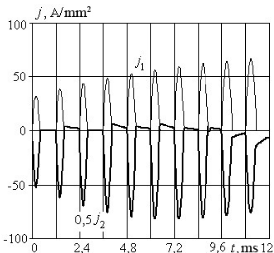
Fig. 3. Electromechanical characteristics of the IDC when excited by a packet of pulses from the CES sections of the same capacitance C_0 = 100 \mu\text{F} , charged to different voltages U_0
