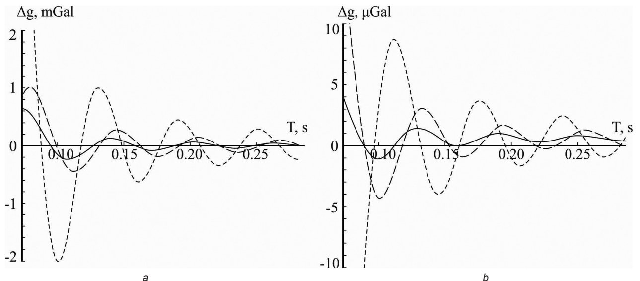
Fig. 5. Auto seismic uncertainty component of g measurement for the BLG without (a) and with (b) vibration protection
