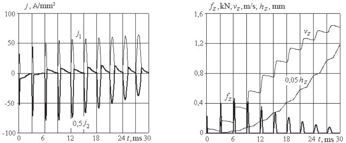
Fig. 4. Electromechanical characteristics of the IDC when excited by a packet of pulses with a period of 3 ms, from the CES sections charged to a voltage U_0 = 210 V, which capacity C_0 increases linearly
