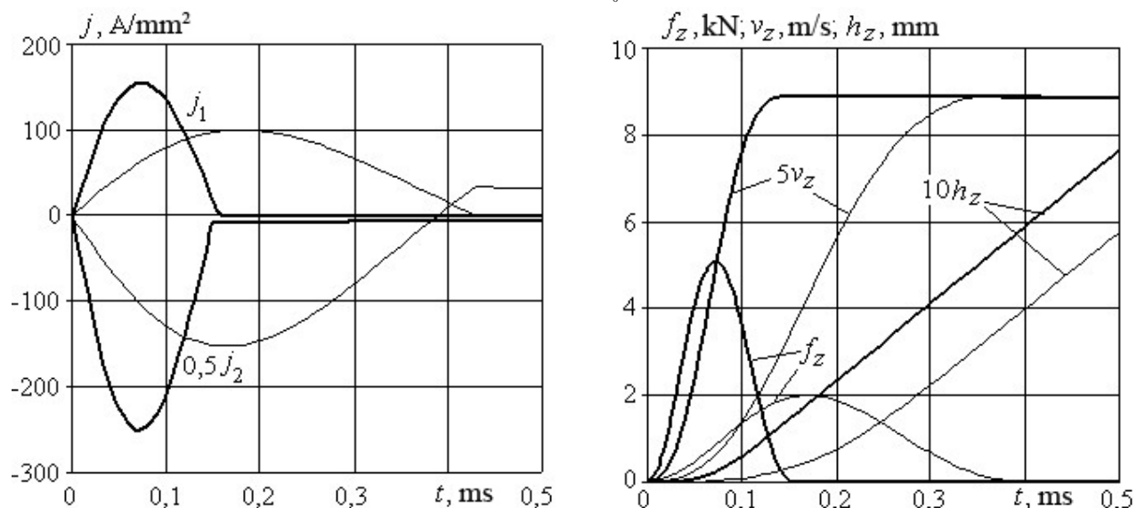
Fig. 1. Electromechanical characteristics of the IDC when excited by a single pulse: variant No. 1 of the CES (bold lines) and variant No. 2 of the CES (thin lines)
