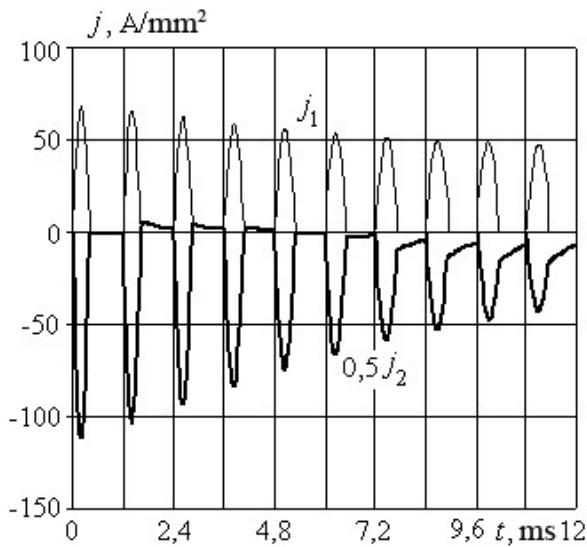
Fig. 2. Electromechanical characteristics of the IDC when excited by a packet of pulses from the CES sections with the same parameters: C_0 = 100 \mu\text{F} , U_0 = 320 \text{ V}
