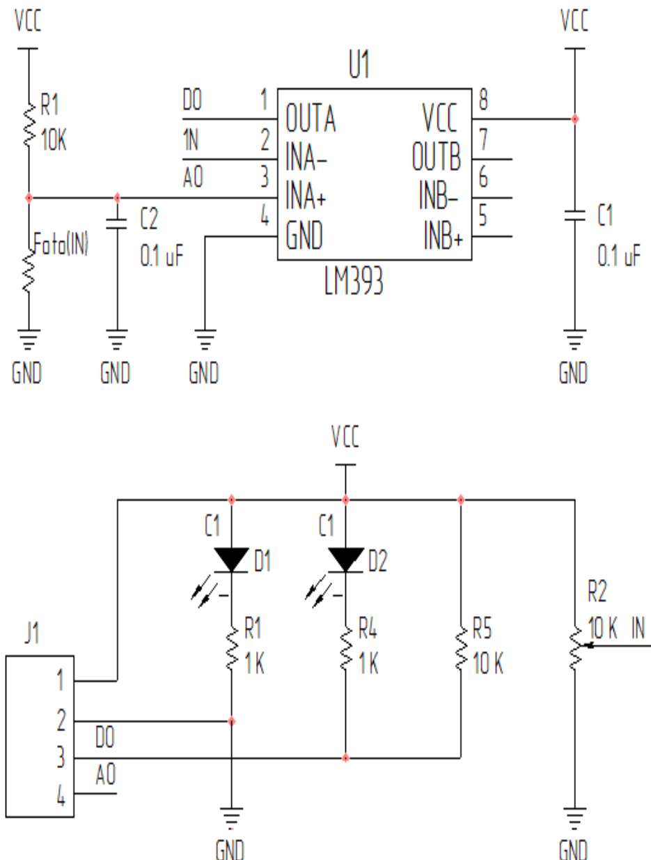
Figure 1: Module schematic diagram
