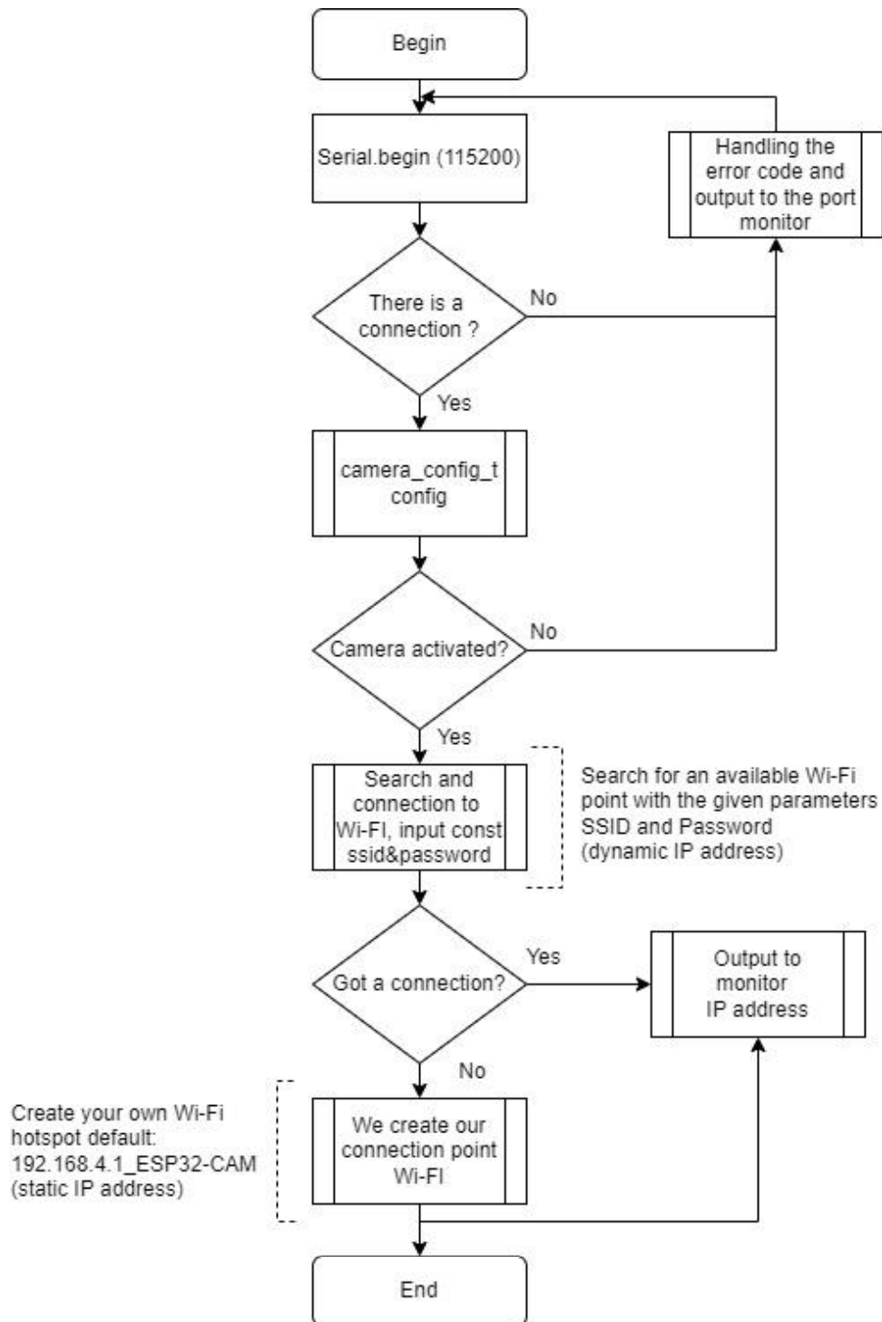
Fig. 1. Enlarged Algorithm for Connecting/Creating of an HTTP server based on ESP32-CAM
