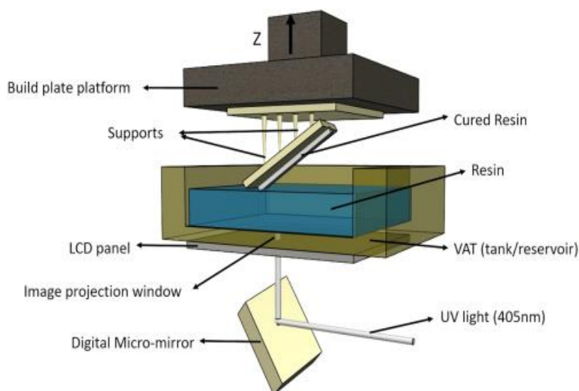
Fig. 5. Scheme of LCD printer operation
