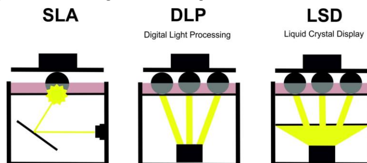
Fig. 2. Types of photopolymer 3D printing technologies
