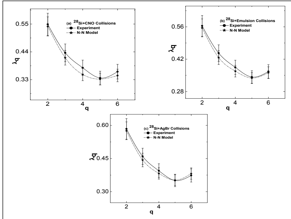
Figure 3 (a-c): Variation of \lambda_q as a function of q for all data sets along with N-N model.
