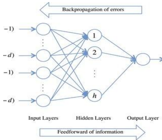
Figure 2: A sketch of multilayer Neural Network (N-N) Model.
