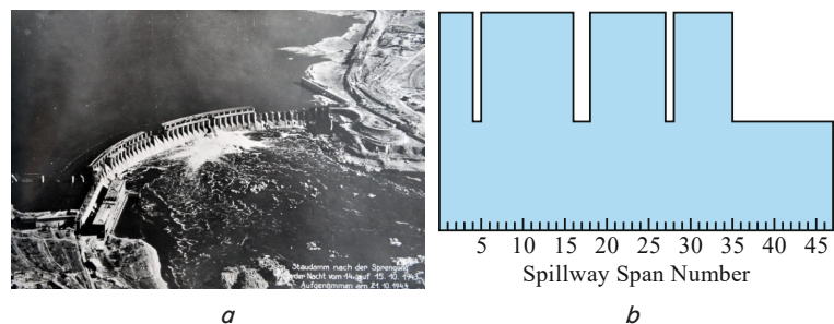
Fig. 11. Dnipro HPP Dam: a – after the explosion on October 15, 1943; b – diagram of destruction of the above-water part of the dam
