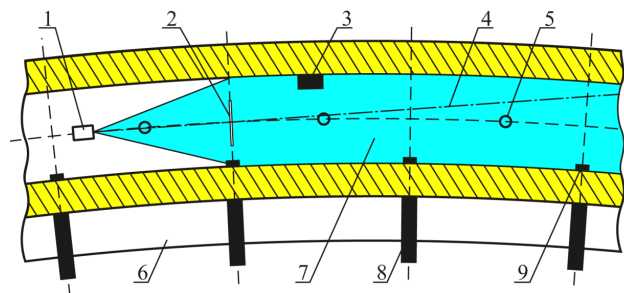
Fig. 4. Scheme of capturing the gallery space by the camera frame due to the structural curvature of the dam (top view): 1 – camera; 2 – large-scale ruler; 3 – electrical distribution equipment; 4 – optical axis of the thermal imager; 5 – lighting equipment; 6 – spans of spillways; 7 – the space captured by the camera frame; 8 – supports of spillway spans; 9 – labels with support numbers
