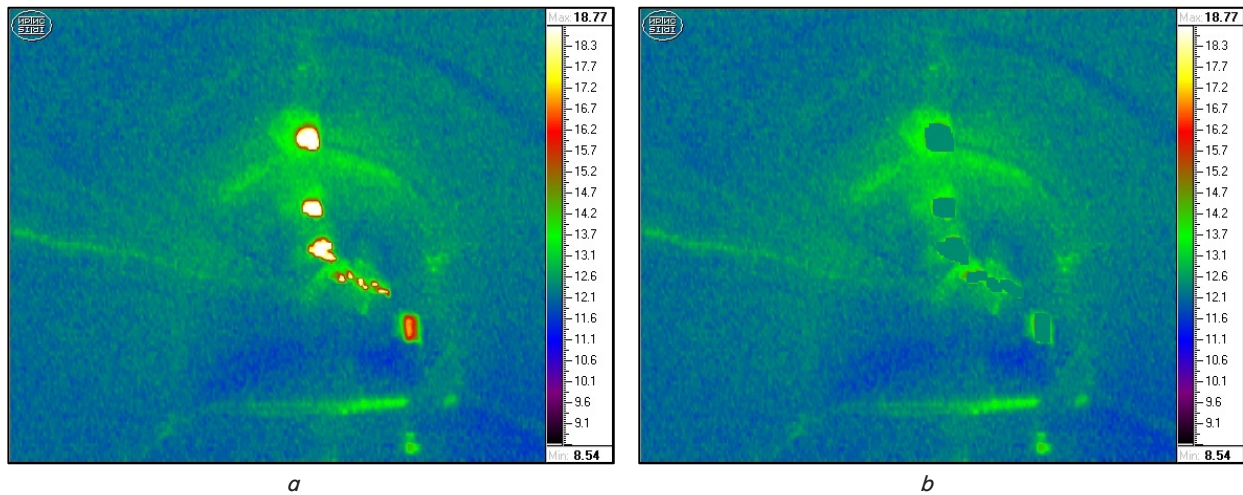
Fig. 7. Eliminating the influence of external sources of radiation: a – initial thermogram; b – processed thermogram
