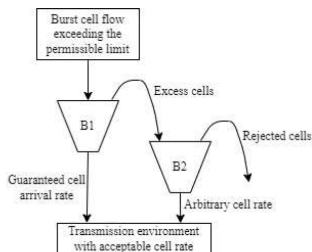
Fig. 3. Physical interpretation of the "leaky bucket" method
