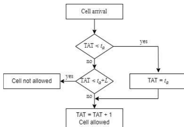
Fig. 2. Virtual scheduling algorithm
