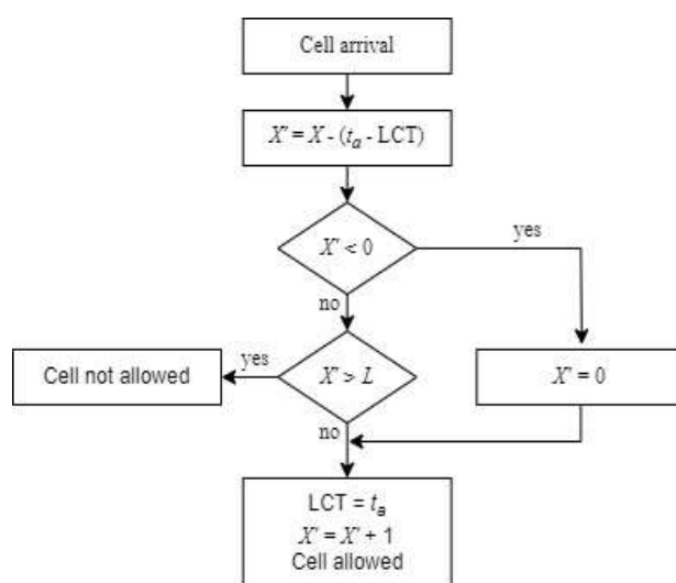
Fig. 4. "Leaky bucket" bitstream control algorithm
