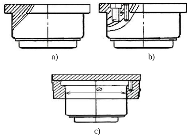
Figure 3: Execution construction scheme of punches designs: a) one-piece punch; b) punch with fastening; c) design of the punch established in a plate-stem holder
