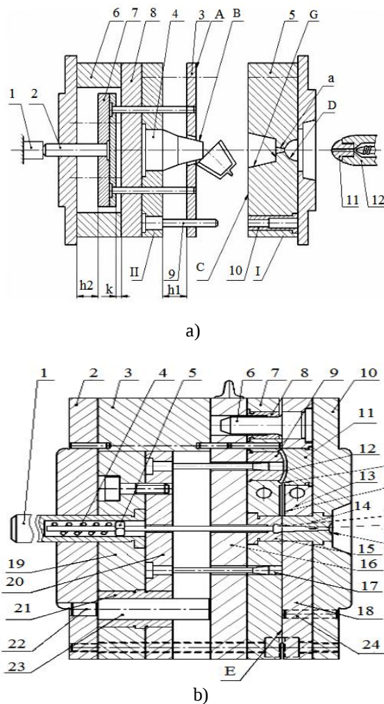
Figure 4: Standard designs of injection molds: a) single-gates form for a "glass" product; b) multiple gates form for a "cover" product
