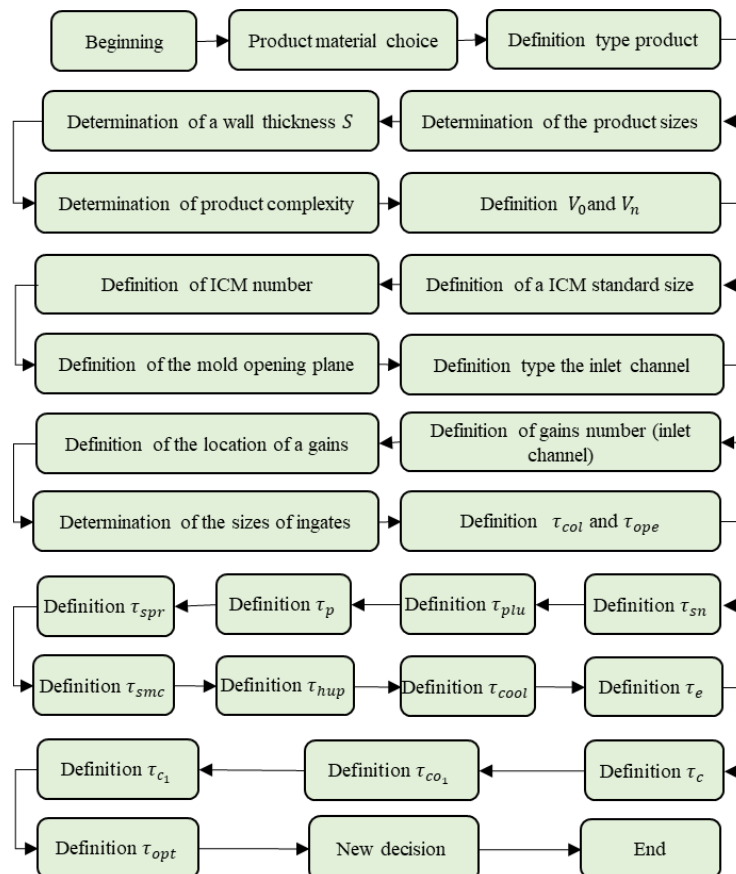
Fig. 4: Flowchart of Decision-Making Process of Time Characteristics Optimization.
