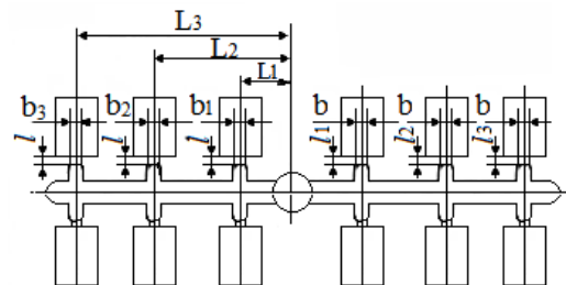
Fig. 3: Balancing Scheme of Inlet Channels.
