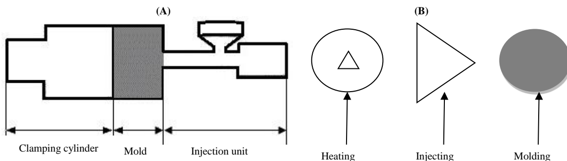
Fig. 1: Injection Casting: a) the Basic Elements of ICP; b) Basic Stages of ICP.
