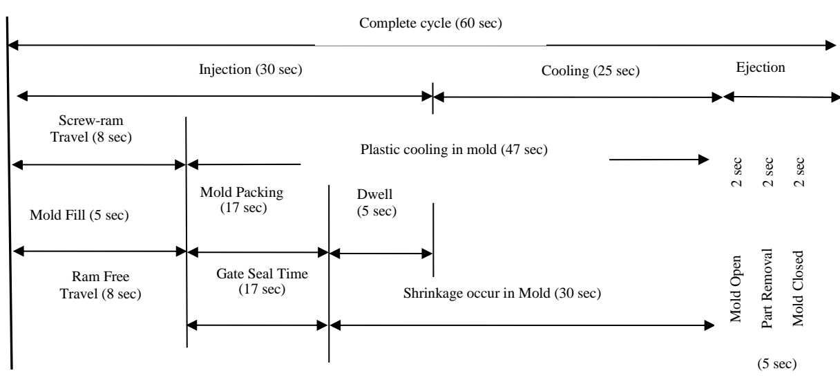
Fig. 2: Example of an Injection Casting Cycle.
