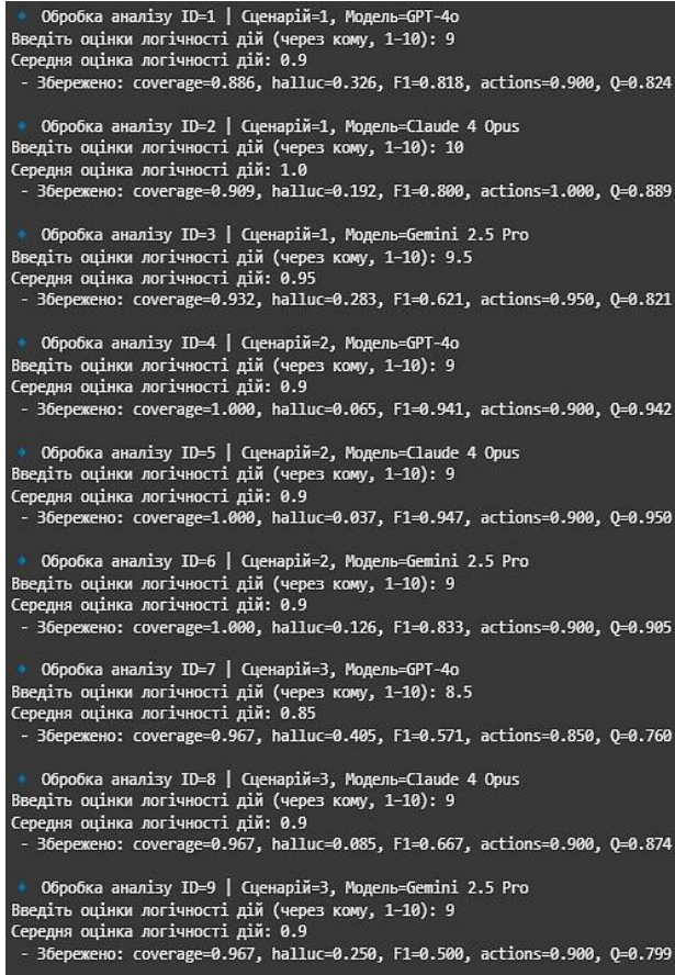
Fig. 5. Calculations of analysis scores for all scenarios
