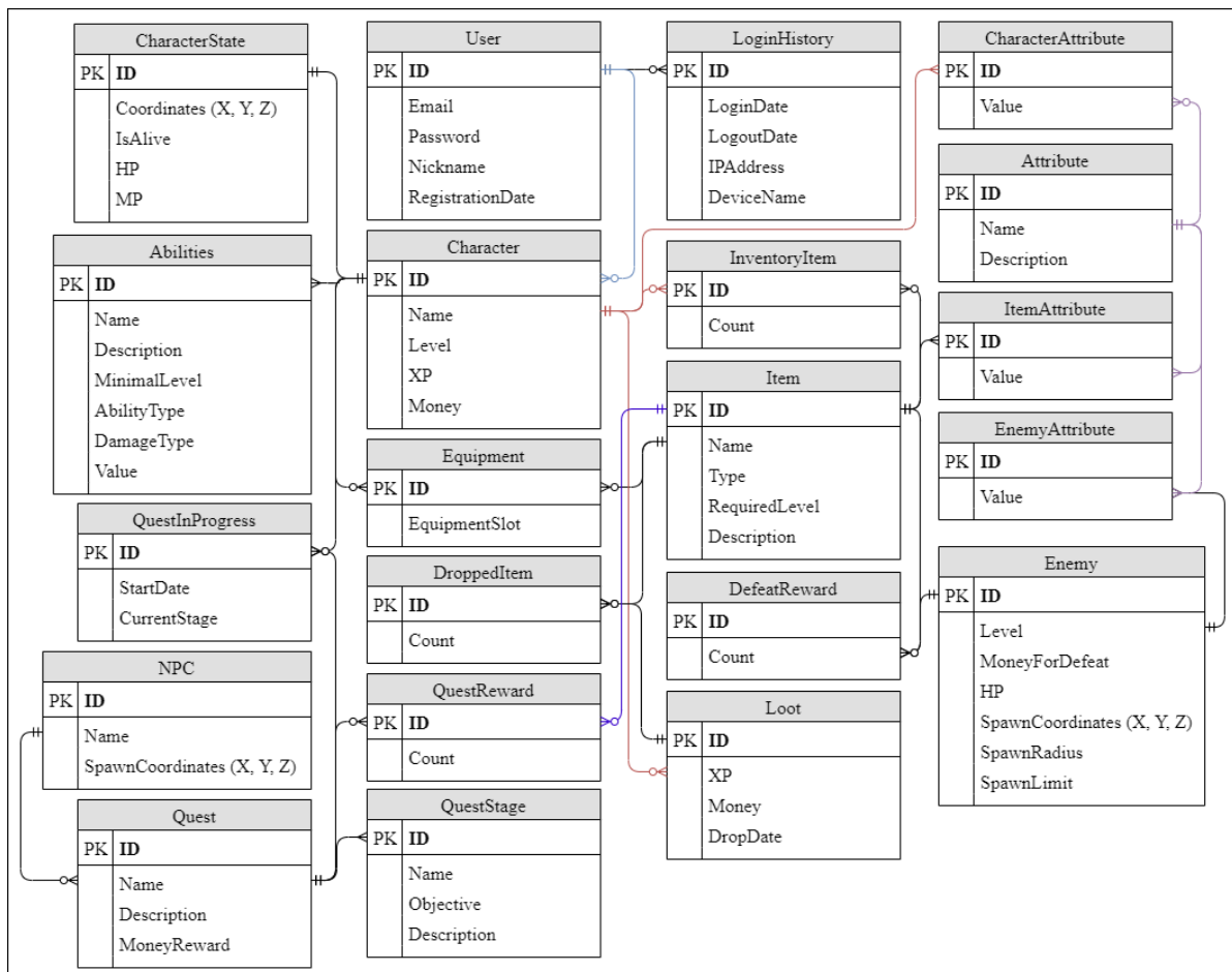
Fig. 4. ER-diagram of the subject area database
