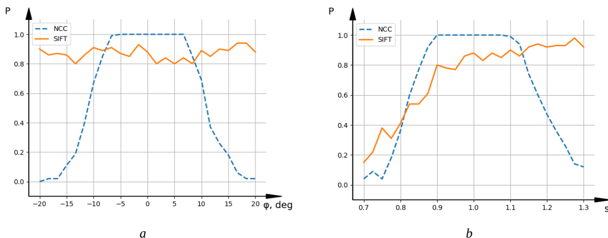
Fig. 6. Probability of correct registration P for small CI (50x50) and RI from Fig. 2, a with respect to: a – rotation \varphi ; b – scale s
