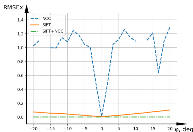
Fig. 7. Effect of rotation \varphi on the RMSE (on X-axis) for the image in Fig. 2, a (similar to Fig. 4, a , with a SIFT+NCC graph)
