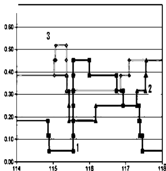
Fig. 9. Dependence of the uplink channel bandwidth on the handover time in the context of the suggested method
