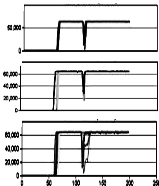
Fig. 10. Channel bandwidth dependence on the handover time
