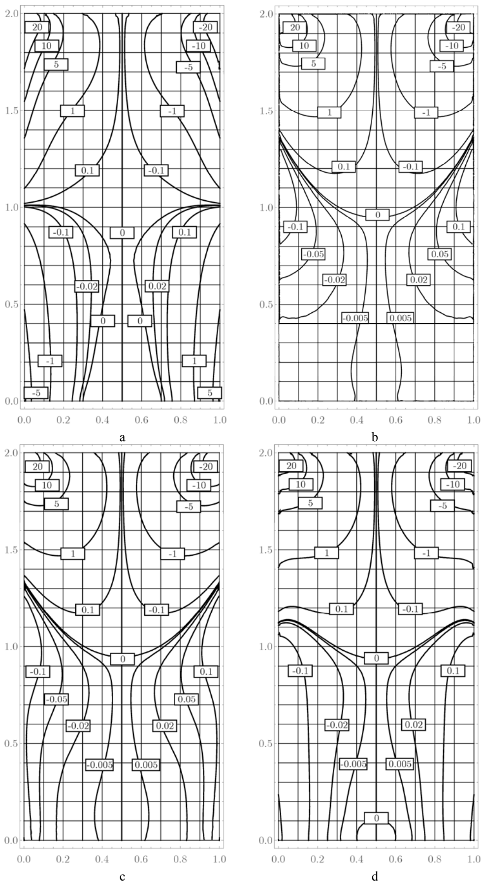
Figure 2 – Pressure contours for the rectangle a = 1 , b = 2 : a - t = 1 , b - t = 3 , c - t = 5 , d - t = 10
