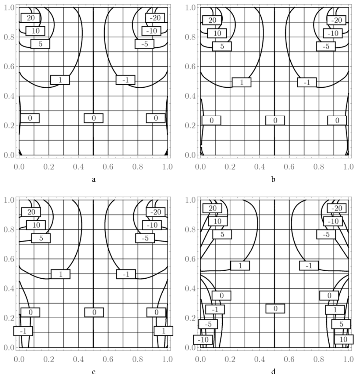
Figure 1 – Pressure contours for the rectangle a = b = 1 : a - t = 1 , b - t = 3 , c - t = 5 , d - t = 10
