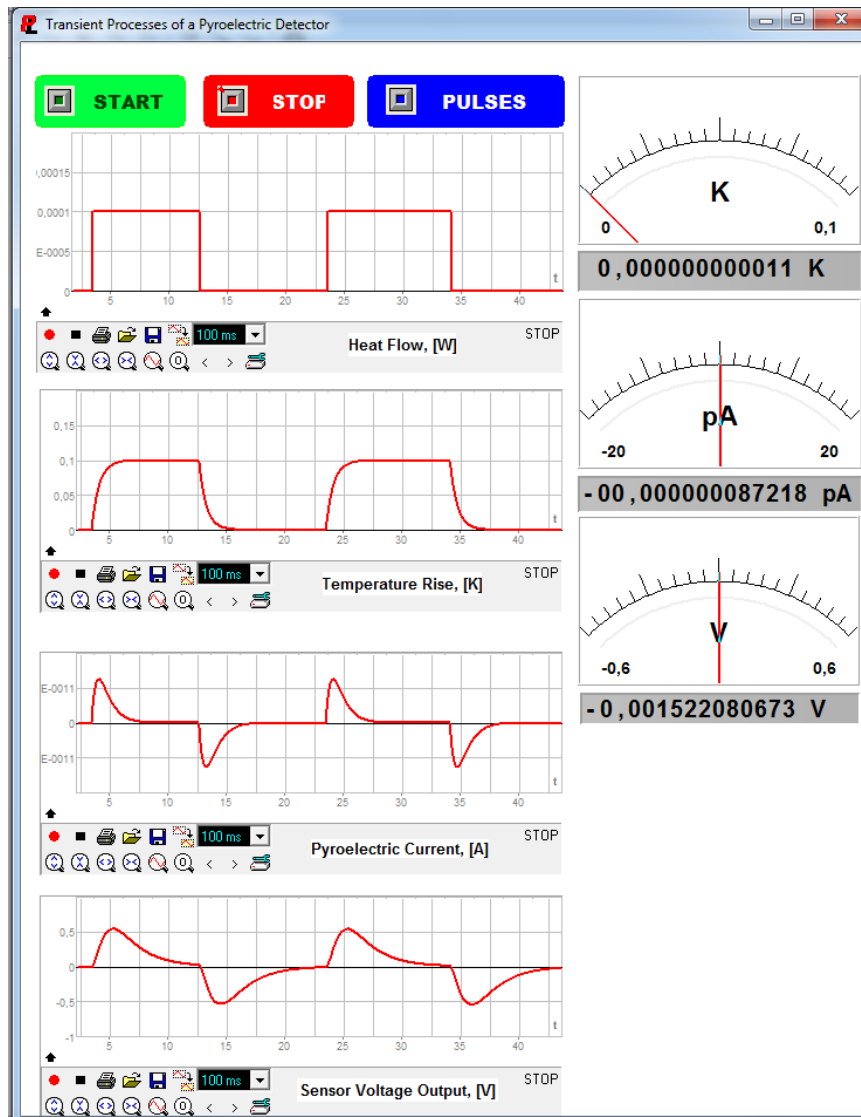
Fig. 1 The simulator for a pyroelectric detector.
