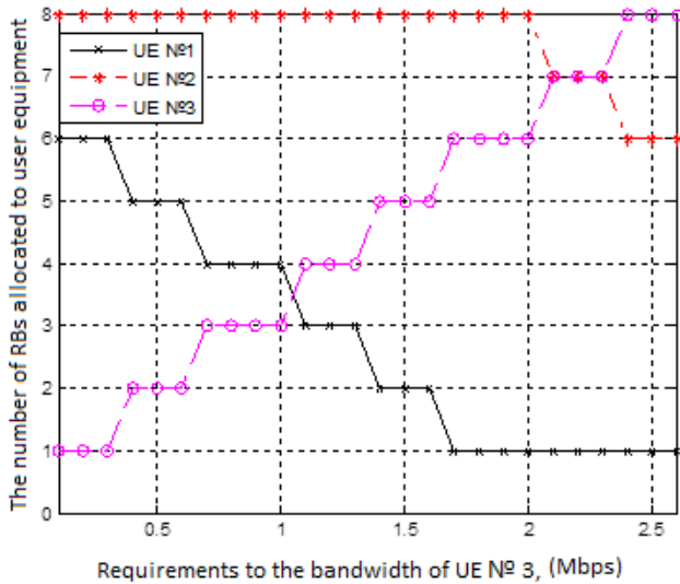
Fig. 7. Dependence of the number of resource blocks allocated to UEs from change of the required bandwidth of the third UE
