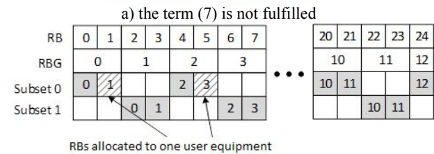
Fig. 4. An example of checking the term (7)
