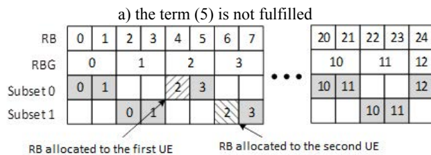
Fig. 2. An example of checking the term (5)
