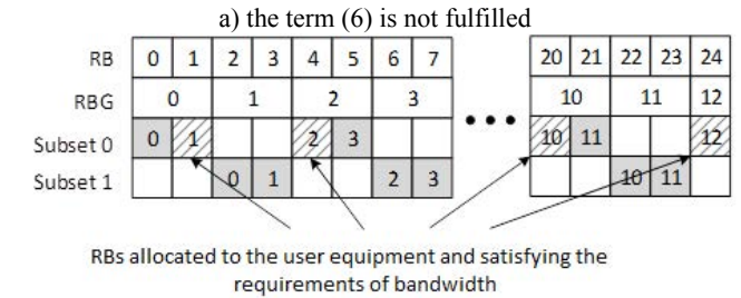
Fig. 3. An example of checking the term (6)
