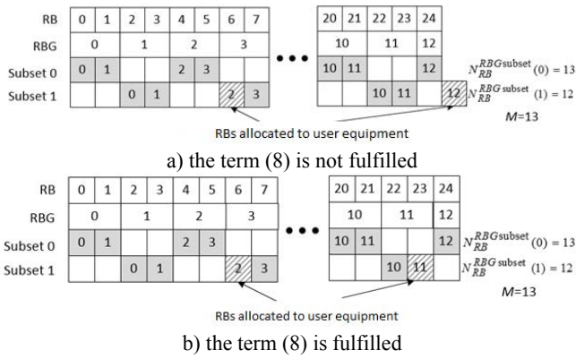
Fig. 5. An example of checking the term (8)
