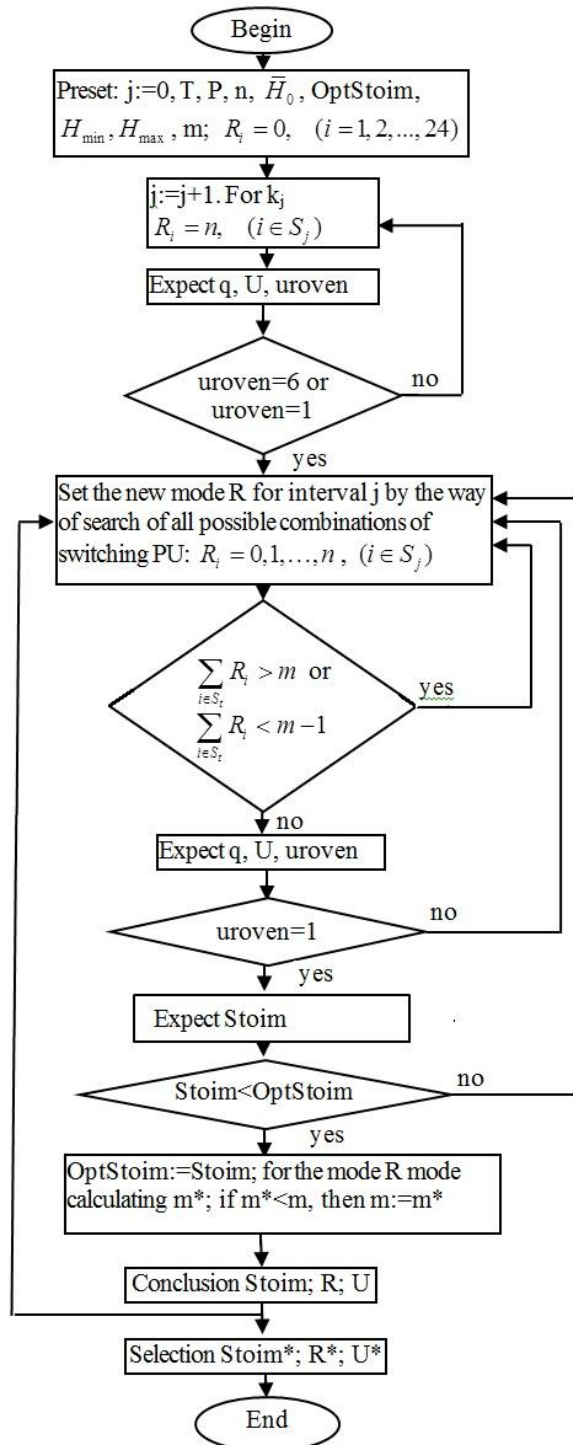
Fig. 3. Flow chart of the algorithm of searching of the optimal mode of operation of SPS at the interval of control [0, T]
