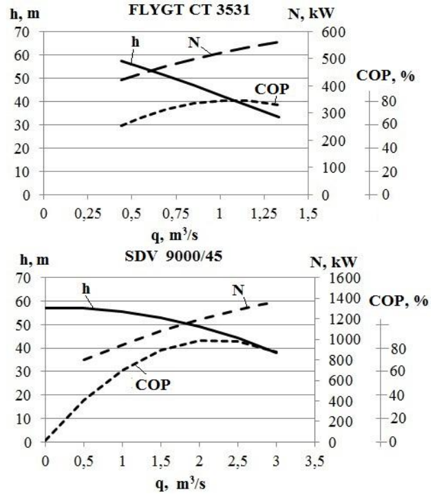
Fig.4. The characteristics of the pump units FLYGT CT 3531 and SDV 9000/45
